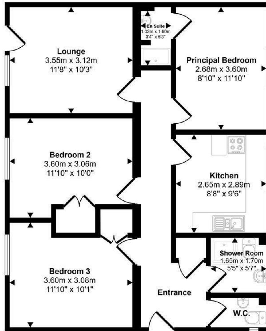
Floorplan
